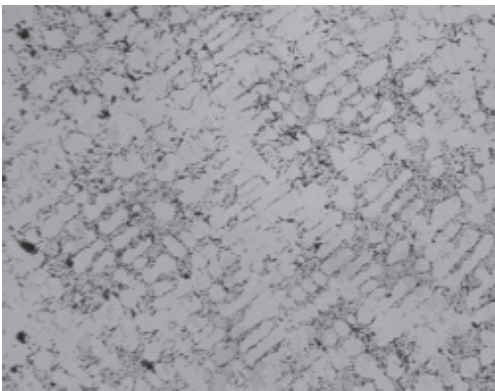
Fig. 2 Type VII flake, type D, size 6-8 (100x, unetched)
