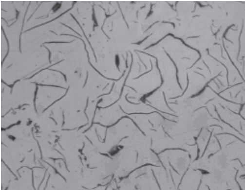
Fig. 1 Type VII flake, type A, size 4-6 (100x, unetched)
