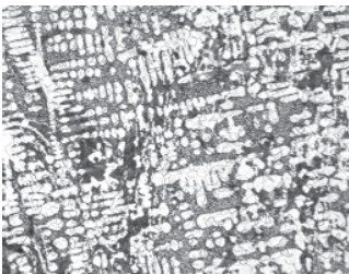
Fig. 4 Typical microstructure in the rim area (100x, etched in 5% Nitrol)
